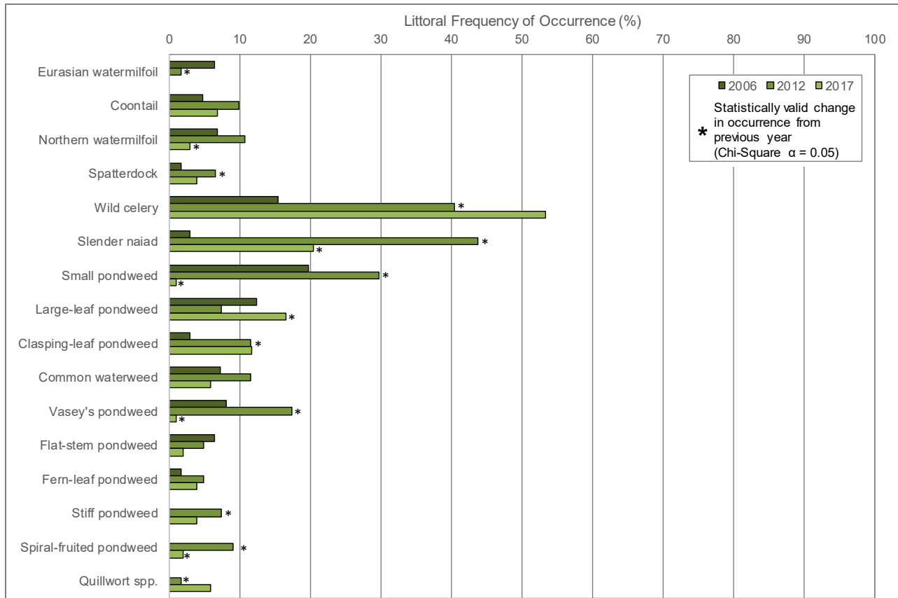
Figure 17. Eagle Lake littoral frequency of occurrence of select aquatic plant species from NEI 2006, Onterra 2012 and 2017 point-intercept surveys. Please note that only those native species with an occurrence of at least 5% in one of the three surveys are displayed. Created using data from 2006, 2012, and 2017 point-intercept surveys.
