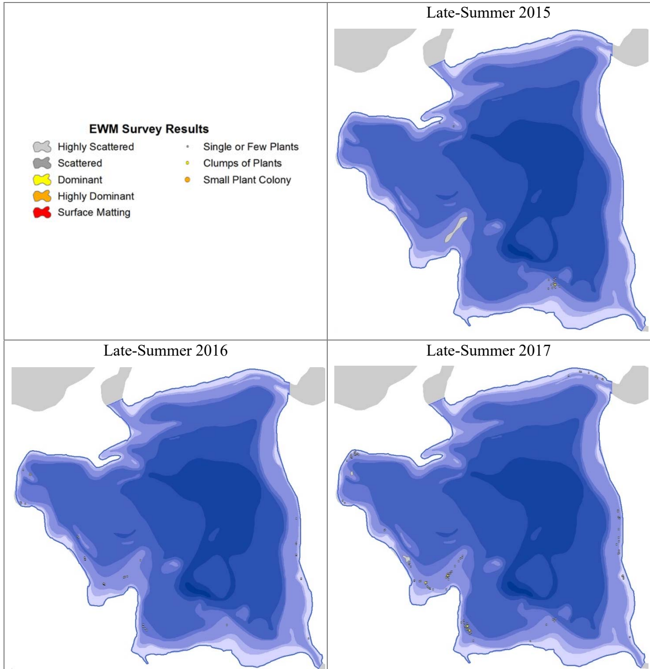
Figure 16. Eagle Lake EWM Population from Late-Summer 2015 to Late-Summer 2017.
