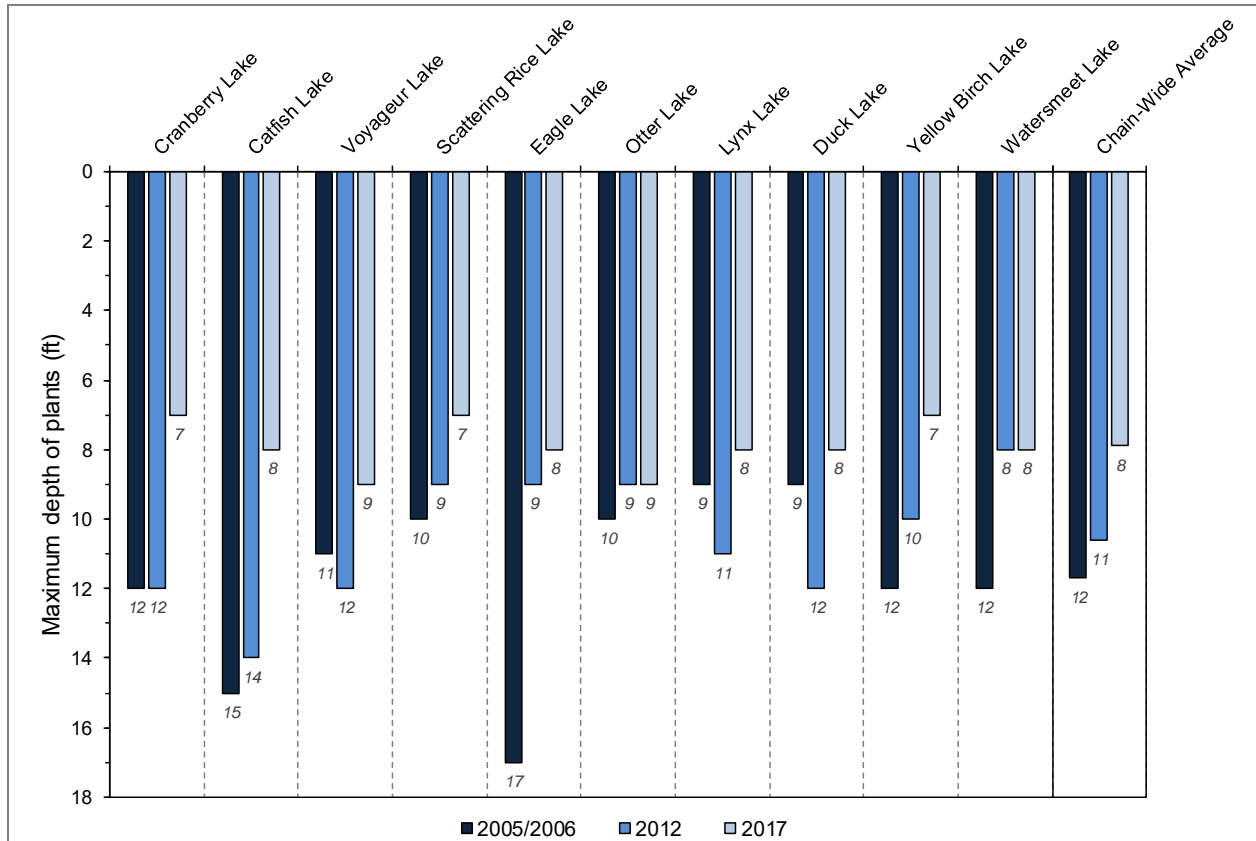
Figure 5. Recorded maximum depth of aquatic plant growth in the Lower Eagle River Chain of Lakes from 2005/06, 2012, and 2017. Decline in maximum depth of aquatic plant growth is due to reduction in chain-wide water clarity over this period.
