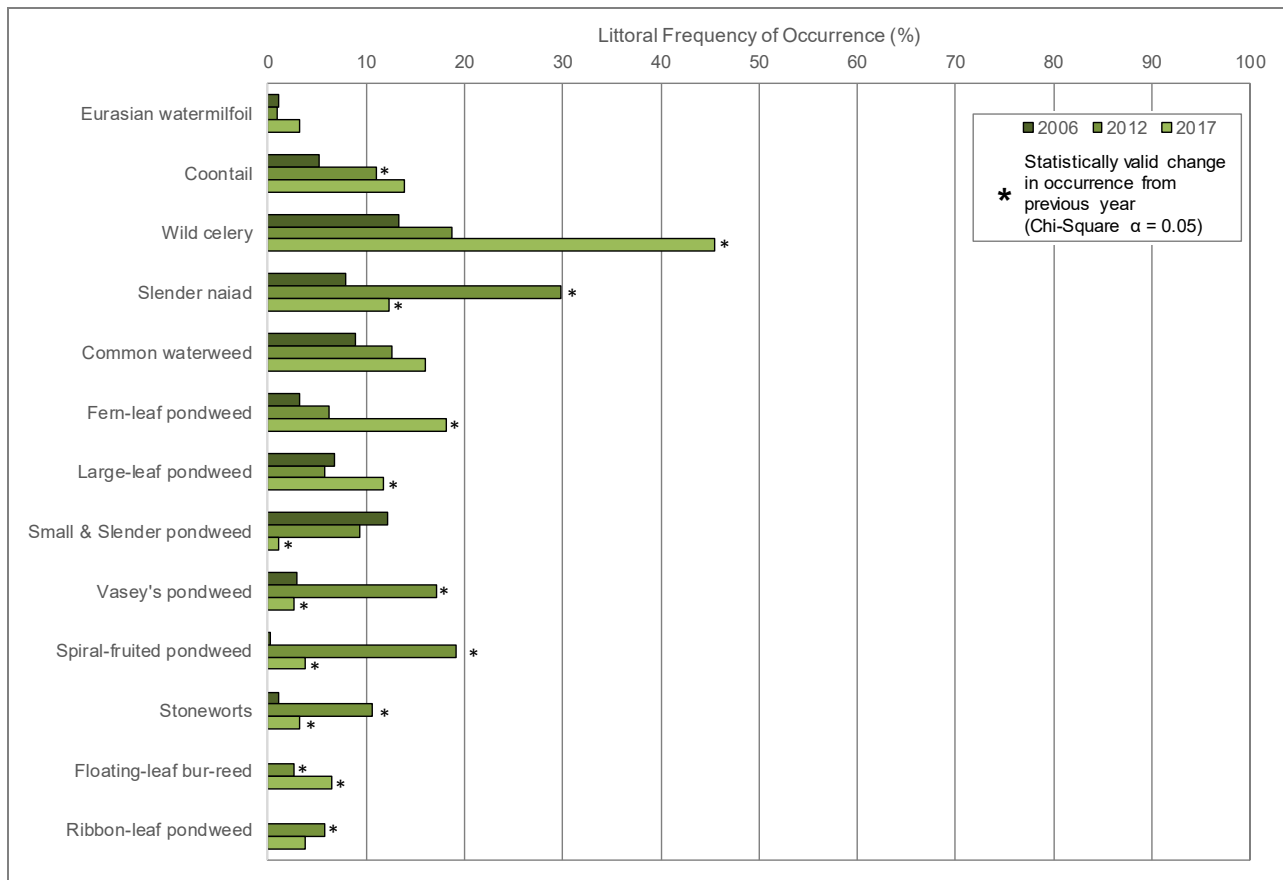
Figure 10. Cranberry Lake littoral frequency of occurrence of select aquatic plant species from NEI 2006, Onterra 2012 and 2017 point-intercept surveys. Please note that only those native species with an occurrence of at least 5% in one of the three surveys are displayed. Created using data from 2006, 2012, and 2017 point-intercept surveys.
