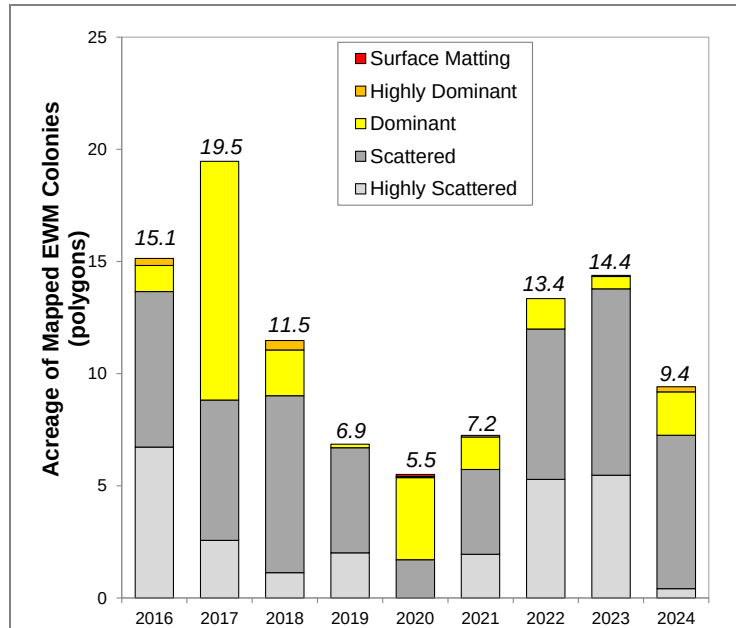
Figure 4.10-1. Watersmeet Lake acreage of mapped EWM colonies during 2016-2024 Late Season EWM Mapping Surveys.
